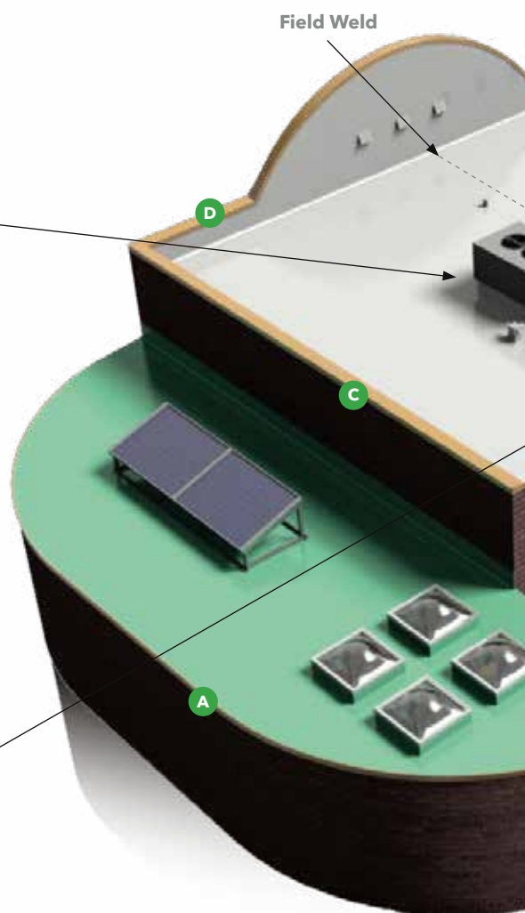
Custom-Fabricated Curb Flashing
